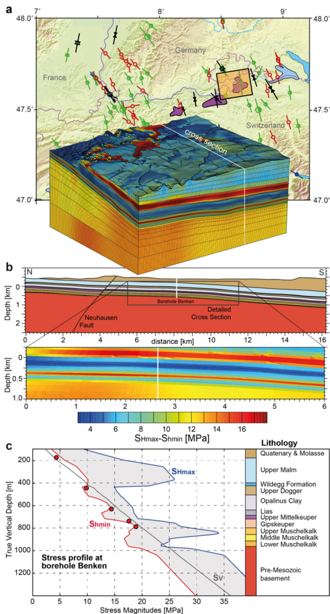
Fig. 8. a) Stress map of northern Switzerland with locations of potential deep geological repository for high-level radioactive waste (purple areas) and extent of the model area (yellow square). 3-D model shows the 20 \times 20 \times 3 \text{ km}^3 model volume with the discretization into finite elements (two-fold vertical exaggeration). Colours show the modelled difference between maximum and minimum horizontal stresses S_{Hmax} - S_{Hmin} (Hergert et al., 2015). White lines indicate the location of the cross section. b) Upper figure shows on a NS cross section the lithological layers within the sediment sequence of the Alpine Foreland that are represented in the model. Lower figure shows the model results of horizontal stress difference S_{Hmax} - S_{Hmin} . c) Modelled magnitudes of S_v , S_{Hmax} and S_{Hmin} along a vertical borehole profile. Red dots show measurements of the S_{Hmin} magnitude in clay rich layers from hydraulic fracturing tests (NAGRA, 2001) that were used for model calibration. Grey shaded area denotes the horizontal stress difference S_{Hmax} - S_{Hmin} . Note that this is only one simulation amongst a wide range of possible solutions that fit the constraints ( S_{Hmin} magnitudes, S_{Hmax} orientation, and stress regime) in this region as well.
