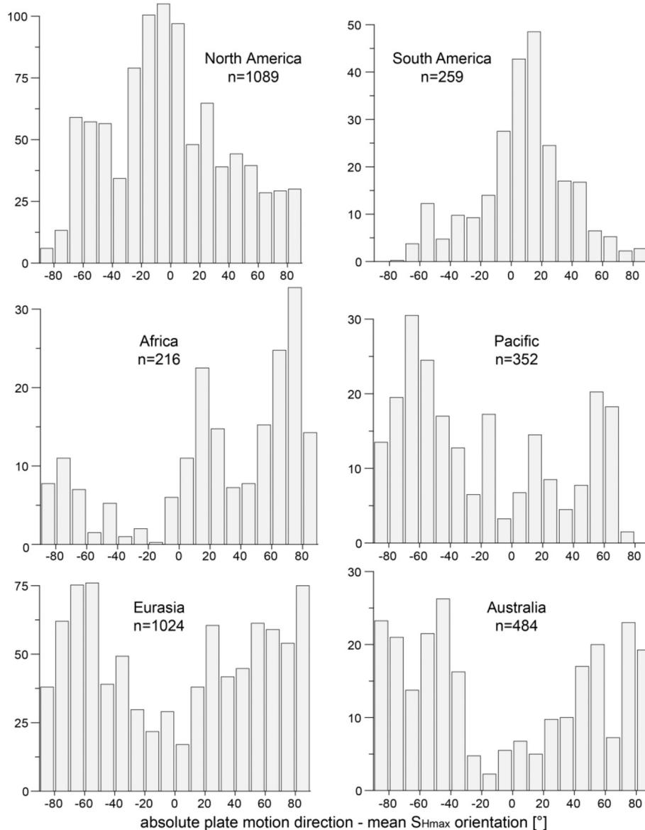
Fig. 5. Deviation between absolute plate motion direction and mean S_{Hmax} orientation. The absolute plate motion direction is estimated from the model HS3 NUVEL-1A (Gripp and Gordon, 2002). For the mean S_{Hmax} orientations the results from a global 1^\circ grid are taken with the same search parameter as stated in Section 3.2. The number n indicates the total number of grid points that returned a mean S_{Hmax} orientation value.
