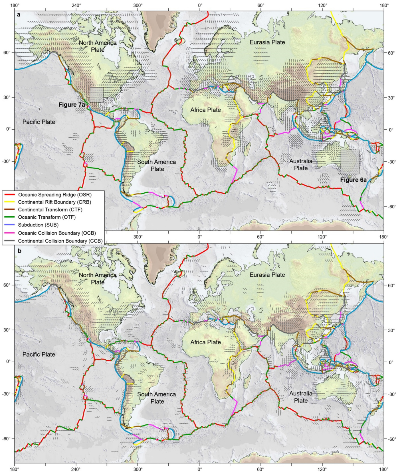
Fig. 4. a) Smoothed global intra-plate stress maps with a fixed search radius of 500 km. Mean S_{Hmax} orientation is calculated on a 2° global grid using A–C quality data without PBE flag. Furthermore, only data records located on the same tectonic plate as the grid point is used to calculate the mean S_{Hmax} orientation. Minimum number of data records within the search radius is n = 5 and data records within a distance of d \leq 200 km to the nearest plate boundary are not used. Plate boundaries are taken from the global model PB2002 from Bird (2003). Furthermore, a distance and data quality weight is applied; the distance threshold is set to 10% of the search radius. b) Same settings as above, but now variable search radii are used. Search radius starts with 1000 km and is decreased in 100 km steps down to 100 km. Mean S_{Hmax} orientation is taken and plotted here for the largest search radius when the standard deviation of the mean S_{Hmax} orientation at the individual grid points is \leq 25^\circ .
