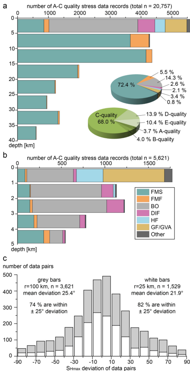
Fig. 3. a) Depth and data type distribution of A–C quality data records and quality distribution of all data records in the WSM database release 2016. FMS: single earthquake focal mechanism, FMF: stress inversion using focal mechanisms; BO borehole breakouts; DIF: drilling induced tensile fractures; HF: hydraulic fracturing; GF: inversion of fault slip data; GVA: geological volcanic alignments. Note that data from FMS and FMF are almost the only stress indicator at depth > 5 km. b) Distribution of data records with A–C quality within the upper 5 km of the Earth's crust. c) Distribution of the deviation of S_{Hmax} orientation from a data record from \leq 5 km depth and the nearest FMS/FMF data record from depth > 5 km within a 100 km (grey) and 25 km (white bars) search radius, respectively. The mean deviation is similar to or smaller than the reliability of the C-quality data (i.e. the S_{Hmax} orientation is reliable within \pm 25^\circ ) indicating that the S_{Hmax} orientation is not varying significantly with depth.
